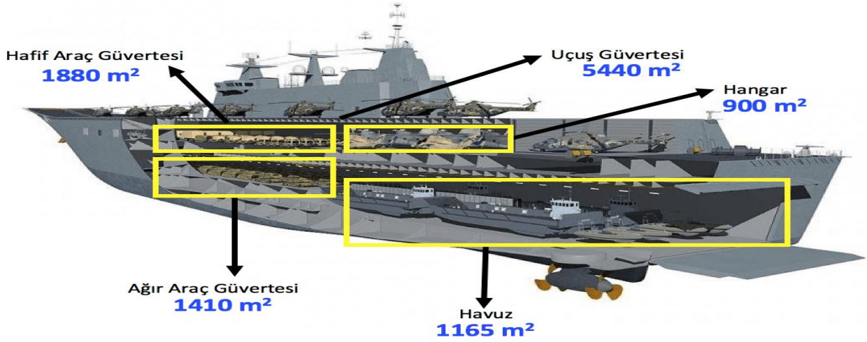
SPS JUAN CARLOS I'in Dikey Kesiti(Durmuş,2018).
